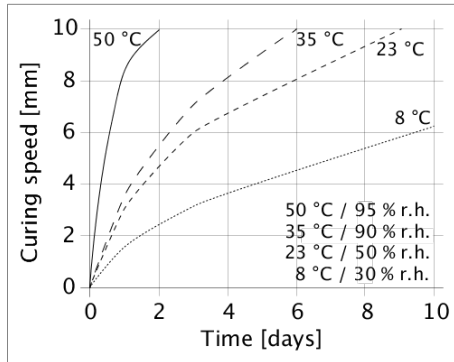
Diagram 1: Curing speed Sikasil® SG-18
