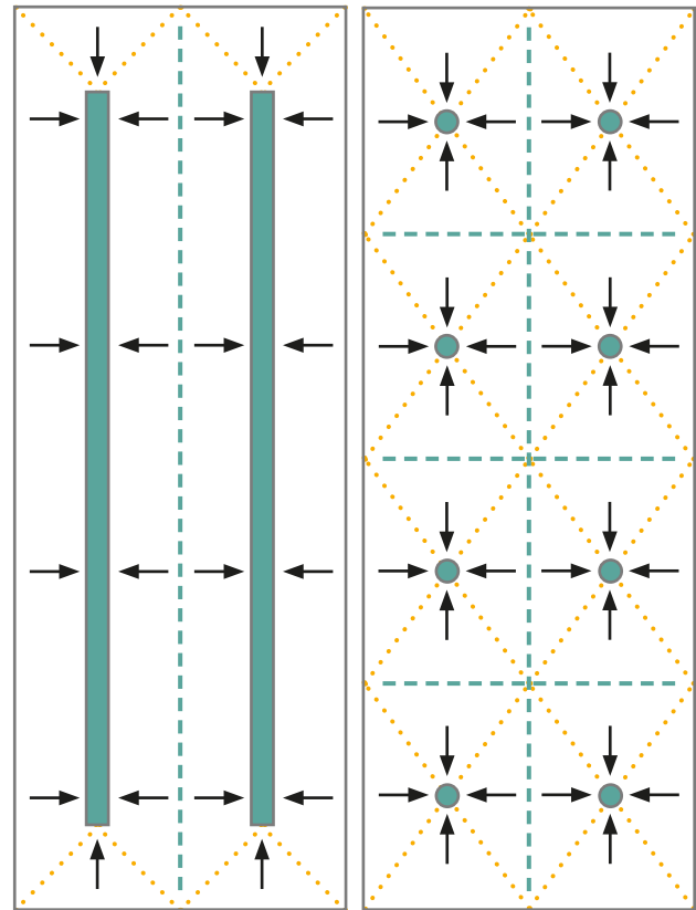
A floor designed with channels (figure on the left) is easier to build than a floor with isolated gulleys (figure on the right).
